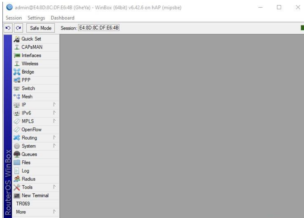
Gambar 1.3 Tampilan Winbox
