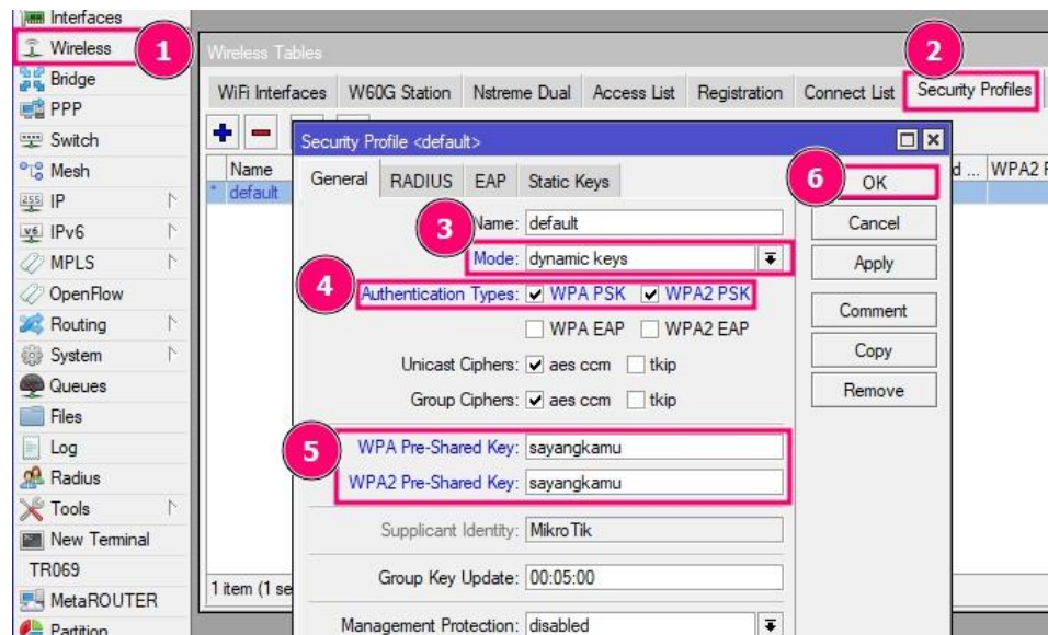
Gambar 1.15 Setting Password
