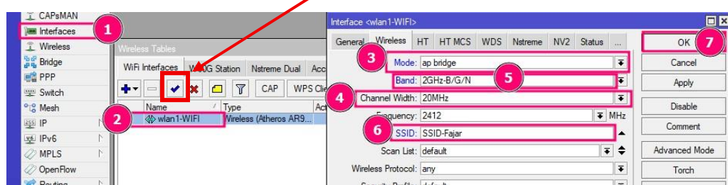
Gambar 1.14 Setting AP Bridge
